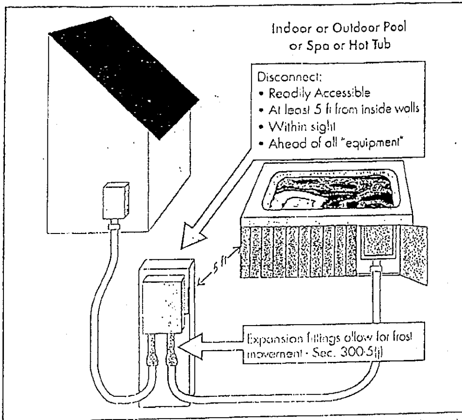
■ Fig. 1.13. A disconnecting means is now intended to be placed within sight of pool, spa, and hot tub equipment.
